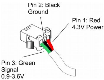
Figure 4: Controller Throttle Pinout
