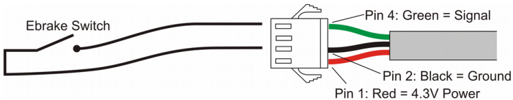
Figure 11: eBrake Connector. 5V+ for Hall Brakes
