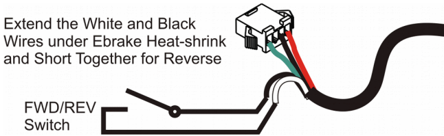
Figure 14: FWD/REV, Remove heatshrink tubing over ebrake connector to expose spare white and black signal wires, and extend those to your reverse switch.
