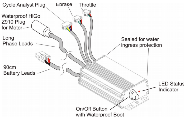
Figure 1: Key Controller Hardware Features
