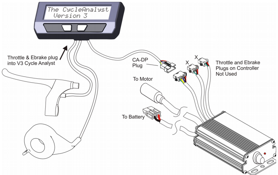
Figure 8: CA V3 Hookup. Throttle and eBrake Plug into CA (not controller)
