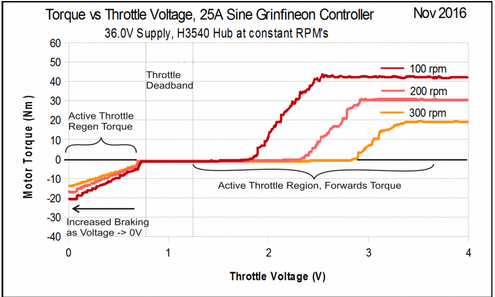
Figure 12: Regen intensity for throttle 0V-0.8V
