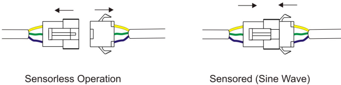
Figure 6: Internal Hall Plug. Inside controller hall wires can be connected or unplugged to change between sensed and sensorless operation
