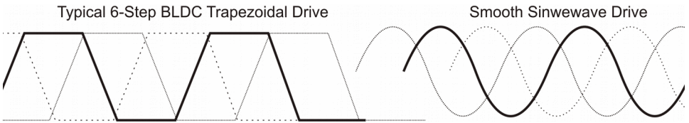
Figure 9: Illustration of Voltage Waveform of Trapezoidal vs Sine Wave Outputs
