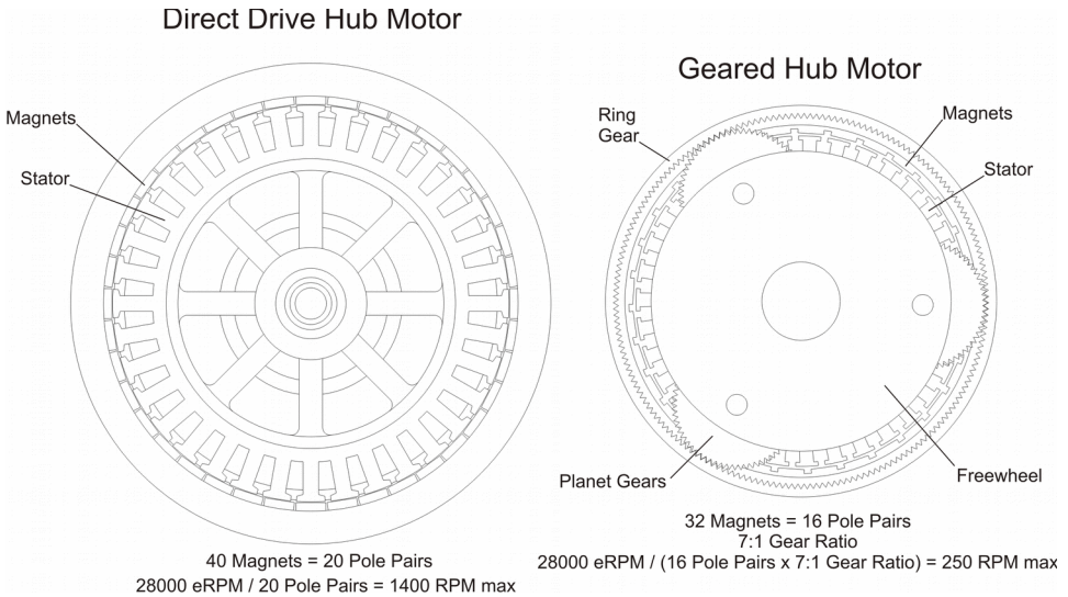
Figure 15: Direct Drive and Geared Hub Motor eRPM examples
