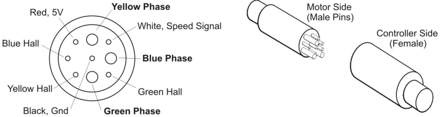
Figure 5: Higo Z910 Controller Pinout (Female Side). The extra white signal wire is used for speedometer line with geared hub motors.
