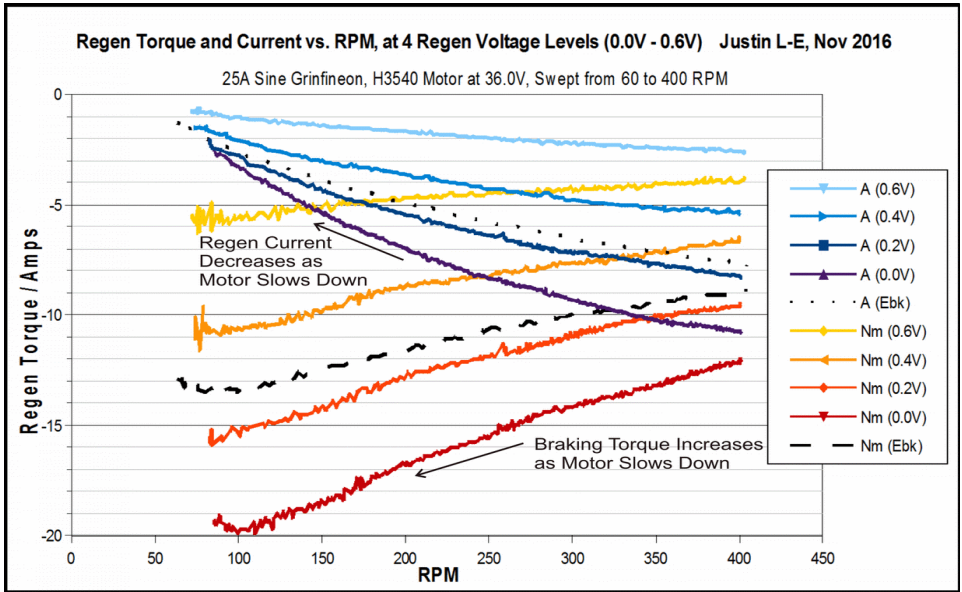
Figure 13: Regenerative Braking Torque and Current as a Function of Motor RPM at 4 different throttle regen voltages and also with ebrake lever pressed (Ebk, dashed lines)
