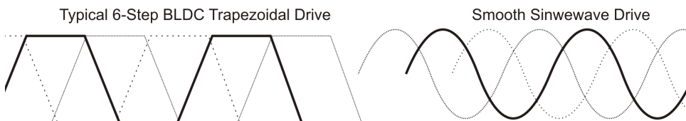
Figure 8: Illustration of Voltage Waveform of Trapezoidal vs Sine Wave Outputs
