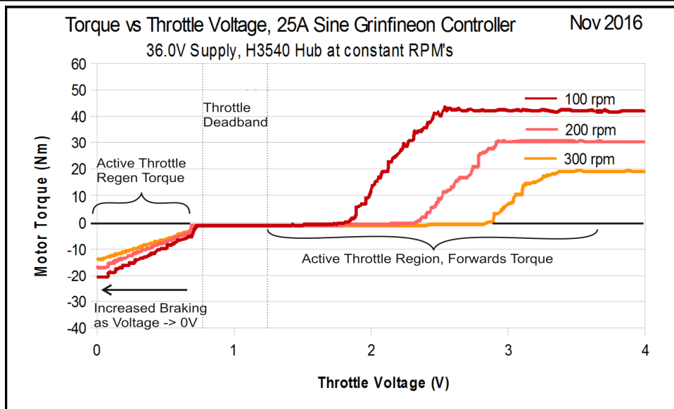
Figure 11: Regen intensity for throttle 0V-0.8V
